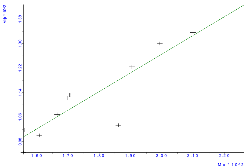
Figure 1. Correlation between the experimental and theoretical values of fabric weight
